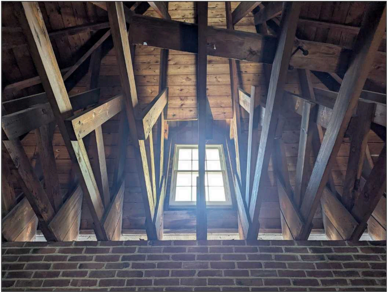
Photo 5: Canoe House roof truss system
